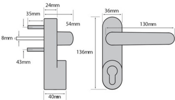
Technical drawing applicable to 83PH36101 & 83PH36102
