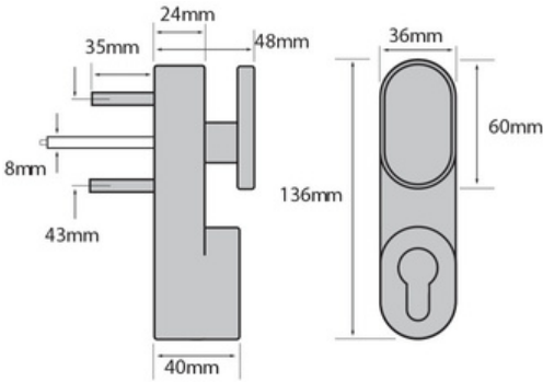
Technical drawing applicable to 83PH37101 & 83PH37102
