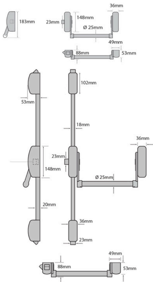
Technical drawings applicable to 83PH3500320, 83PH3550320, 83PH3570320
