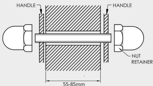
Fixing Kit 2
