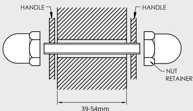
Fixing Kit 1
