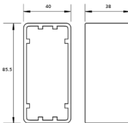
Narrow style surface housing - brushed aluminium
