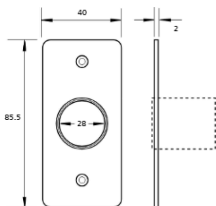
Narrow style plate dimensions
