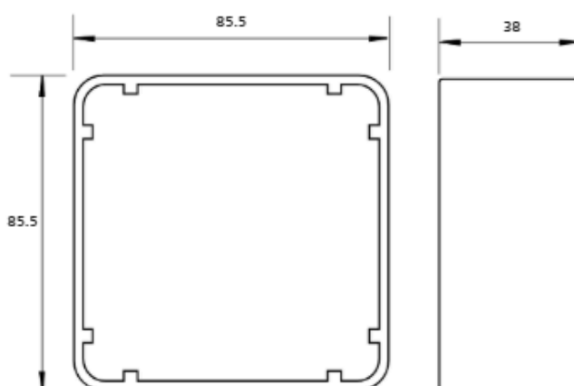
MK1 gang surface housing - brushed aluminium
