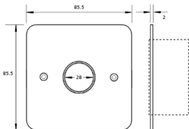
Standard MK1 gang plate dimensions
