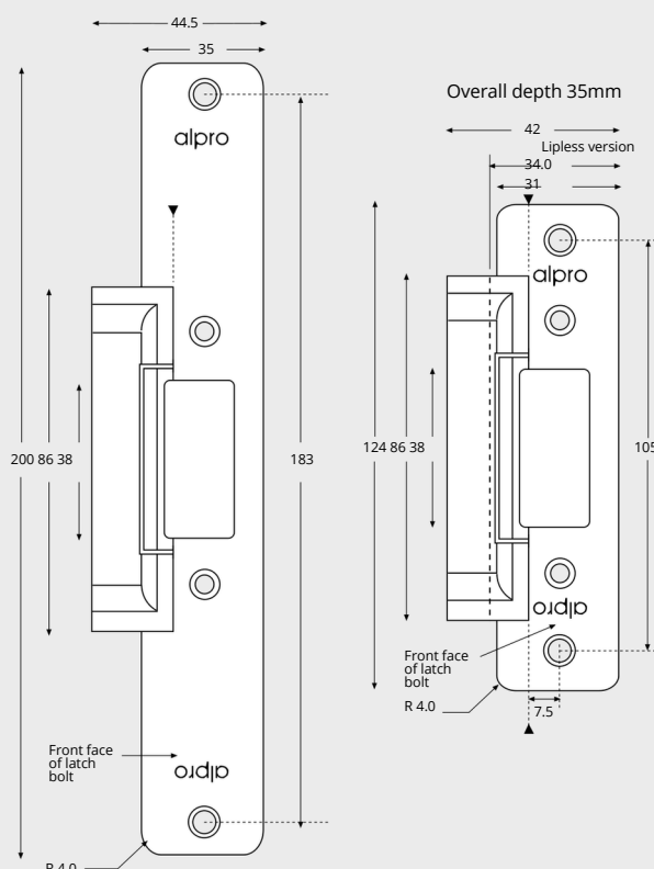
(BS) ANSI Long Faceplate
