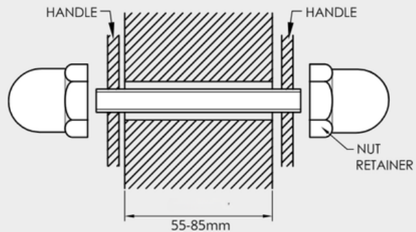
Fixing Kit 2
