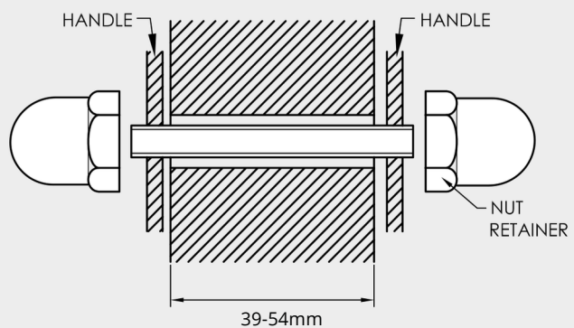
Fixing Kit 1
