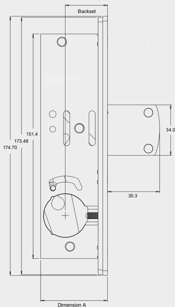
52185 Lock Type
