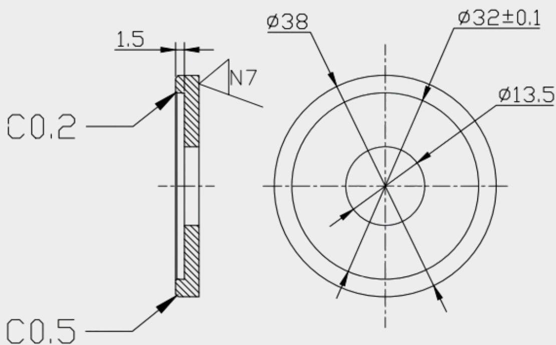
Dimensional drawings shown are for the Rose Fixings
