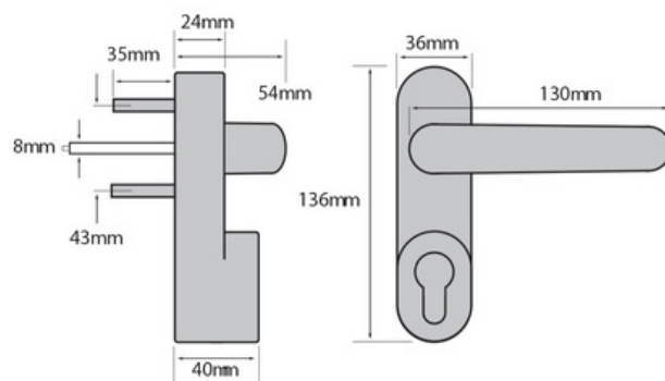
Technical drawing applicable to 83PH3610120
