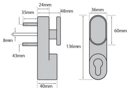
Technical drawing applicable to 83PH3710120
