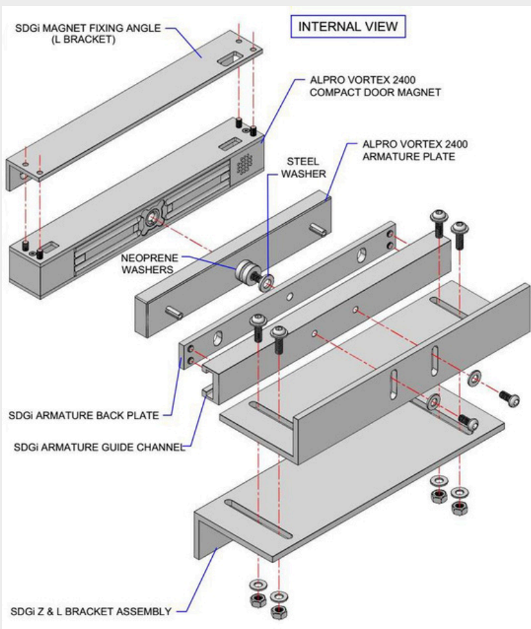
Components and assembly drawing
