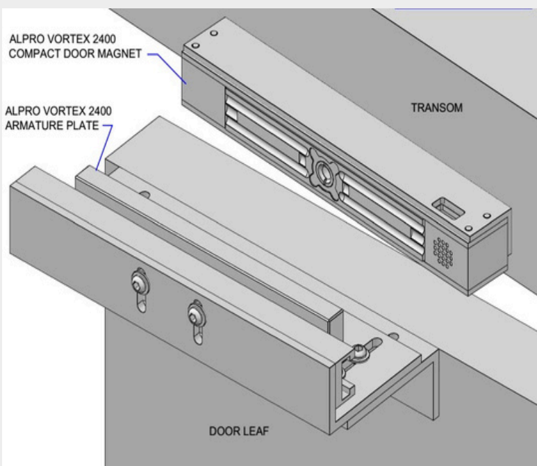
Installed magnet and bracket
